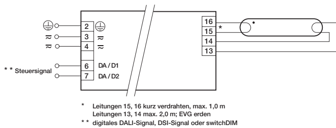
PCA T8 EXCEL one4all Ip x1tec II 1x14–80 W
